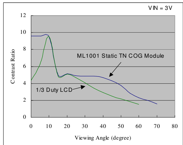
4) Example of Contrast Ratio vs. Viewing Angle
