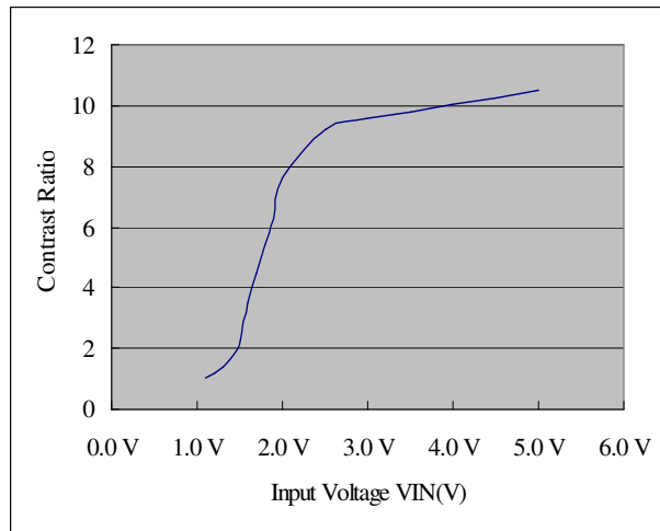
3) Example of Contrast Ratio vs. Input Voltage
