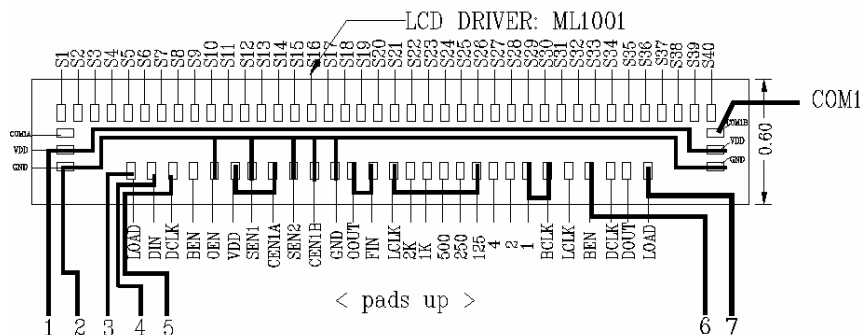
ML1001-1U Application Circuit with 1 Hz Blink Feature
