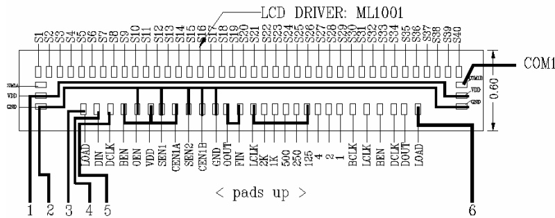
ML1001-1U Standard Application
