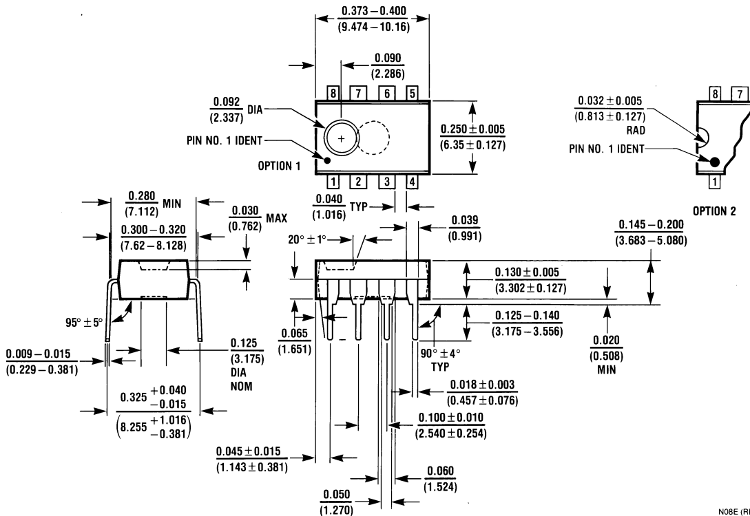
8-Lead (0.300" Wide) Molded Dual-In-Line Package Order Number LM6172IN NS Package Number N08E
