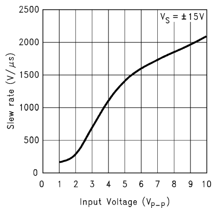
Slew Rate vs. Input Voltage
