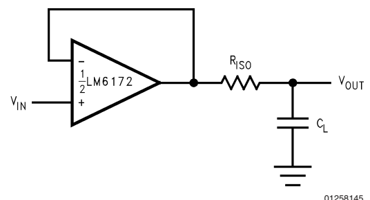
FIGURE 1. Isolation Resistor Used to Drive Capacitive Load
