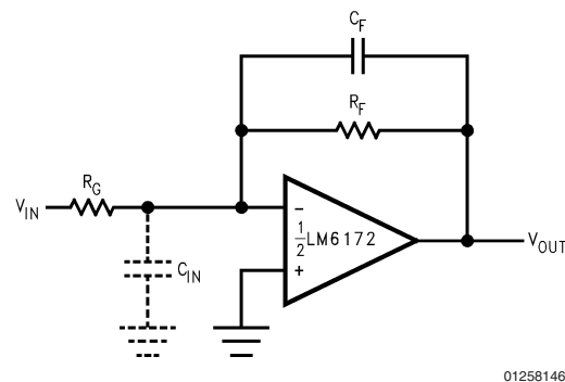
FIGURE 4. Compensating for Input Capacitance
