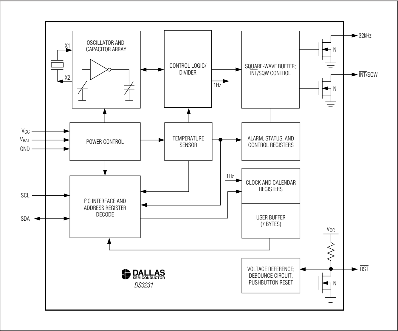
Block Diagram
