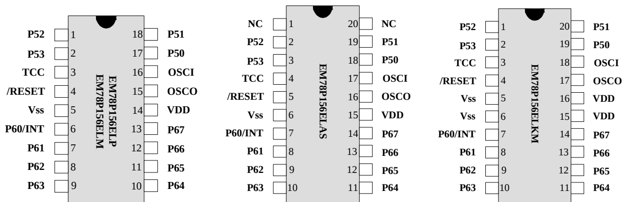
Fig. 1 Pin Assignment
