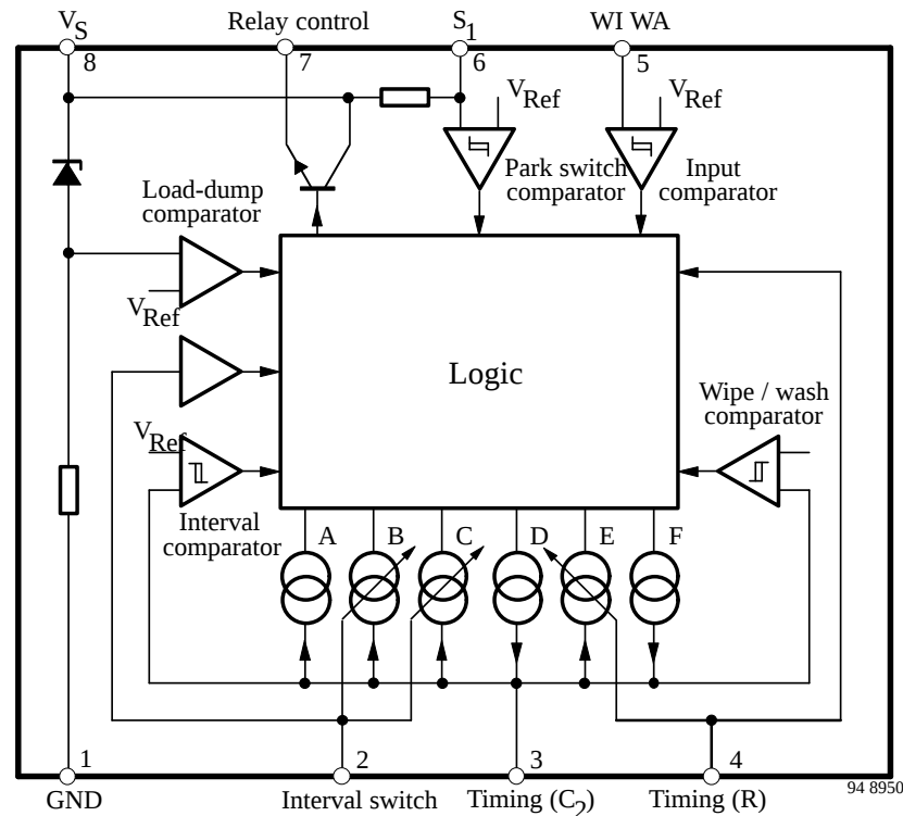
Figure 1. Block diagram
