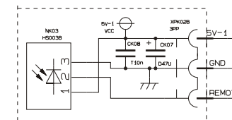
Remote Sensor Board
