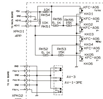
Control Board
