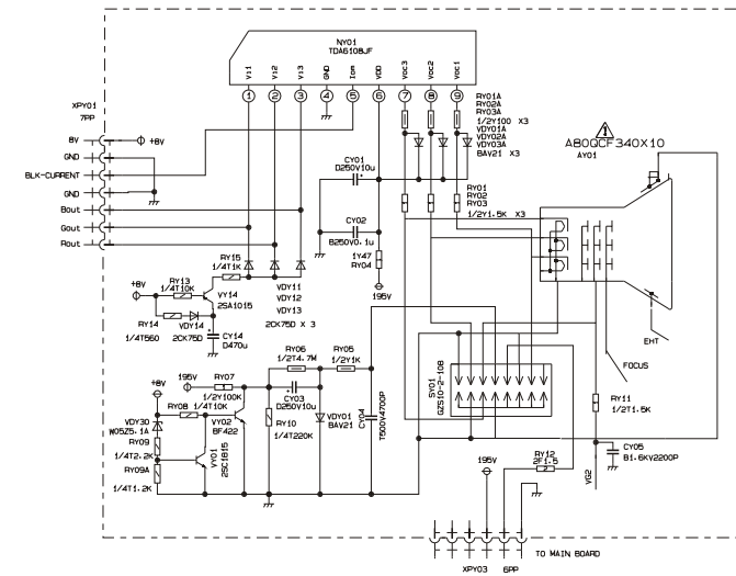
CRT RGB Board
