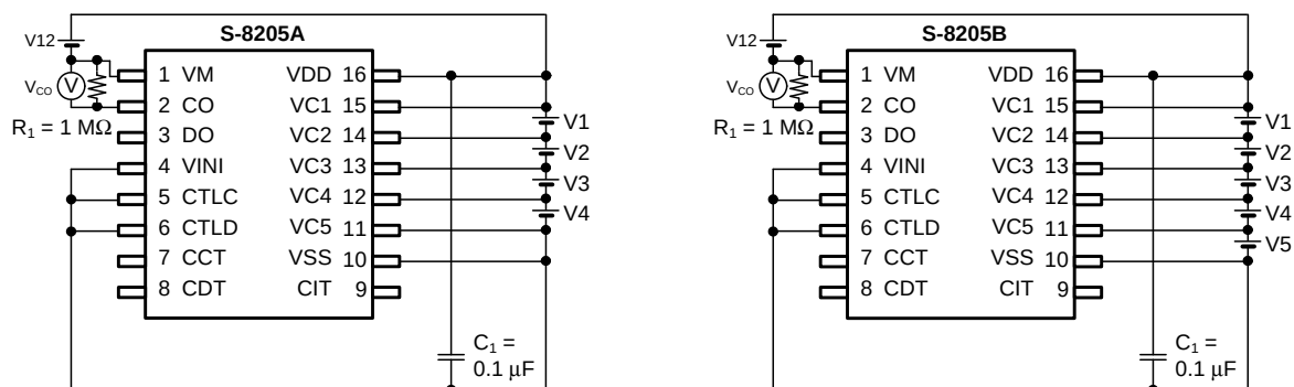
Figure 8 Test Circuit 4
