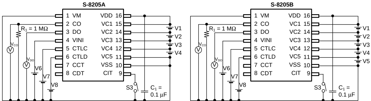
Figure 6 Test Circuit 2
