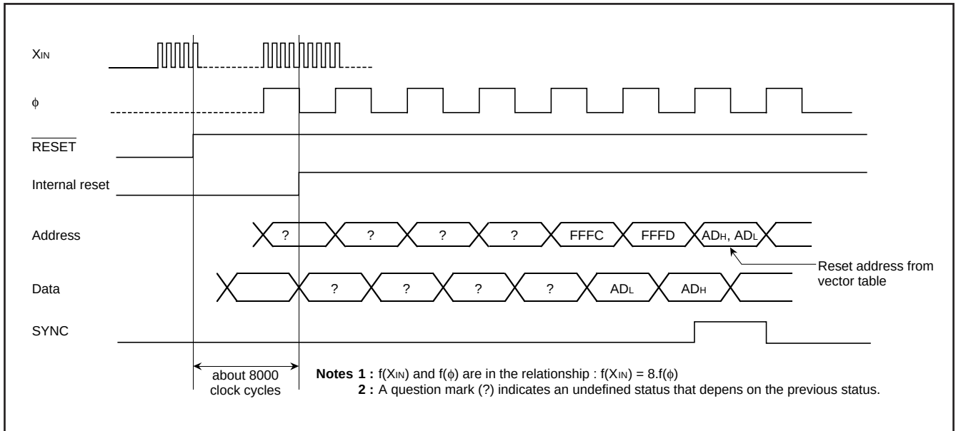
Fig. 28 Reset sequence
