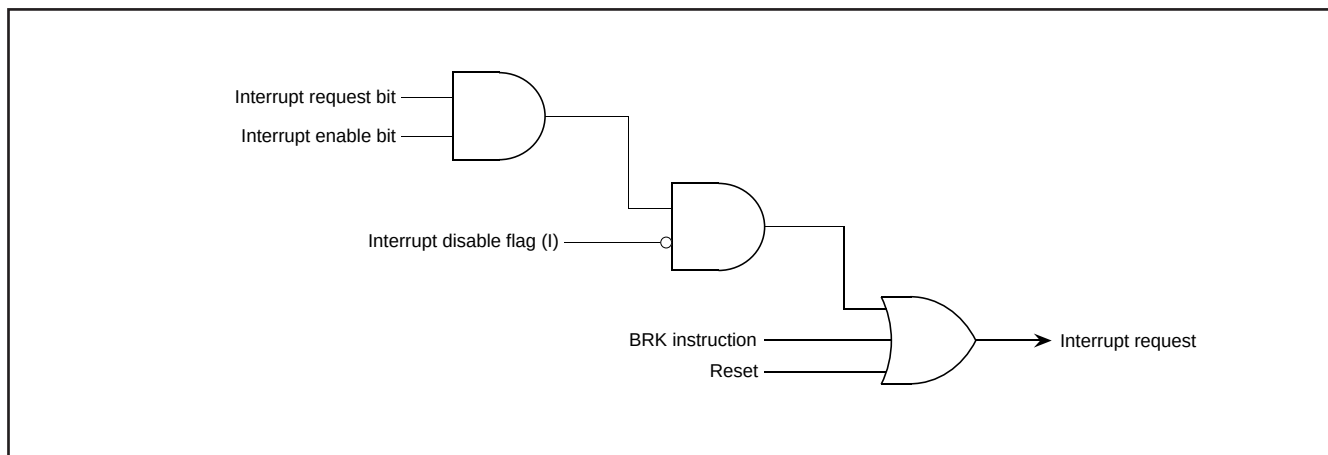
Fig. 7 Interrupt control
