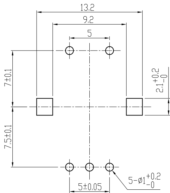
P.C.B.MOUNTING DETAIL
