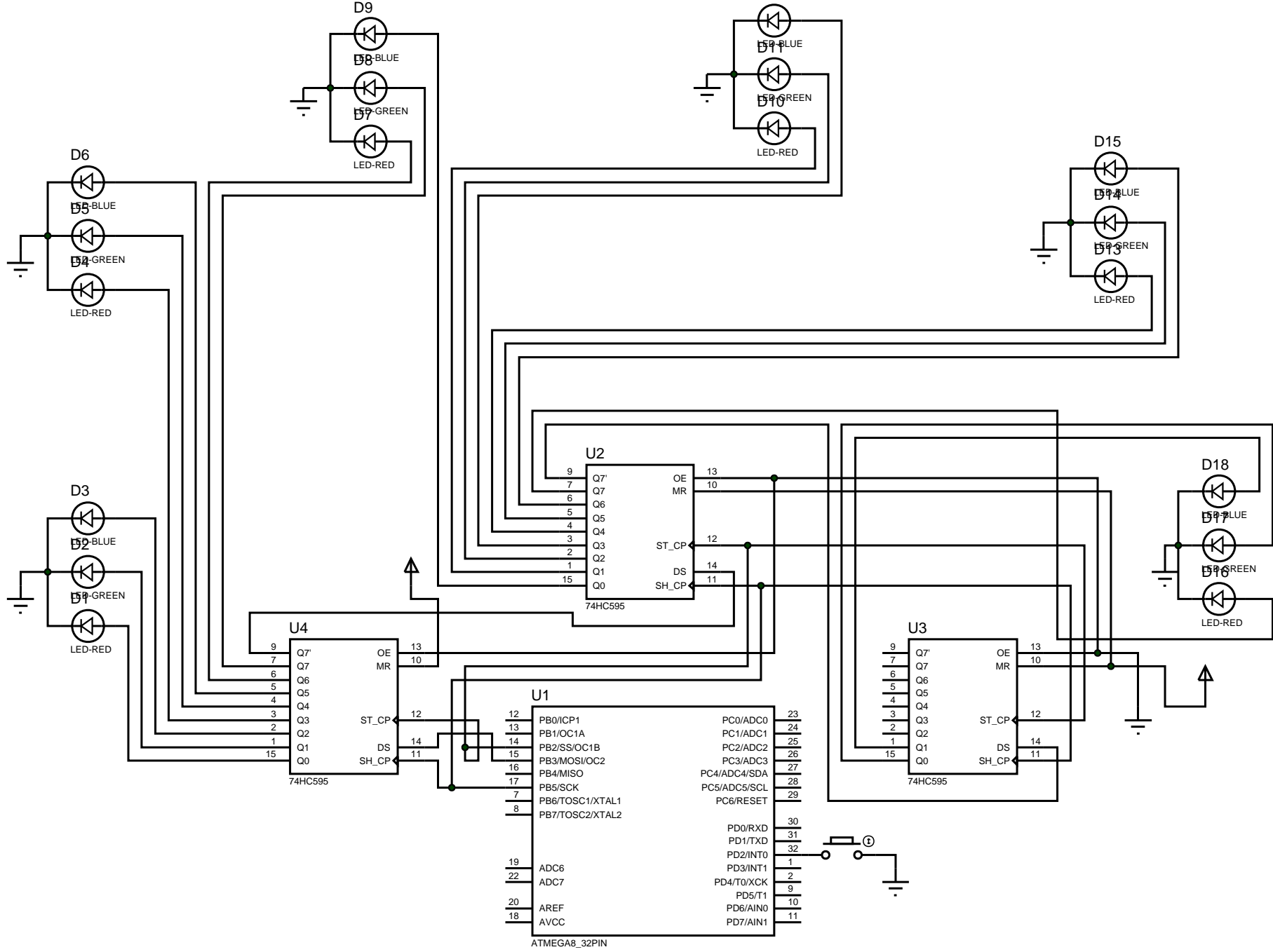
ATMEGA8_32PIN
