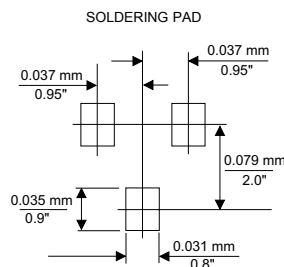
Outline SOT23
