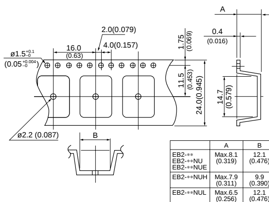
Tape Dimensions Unit : mm (inch)
