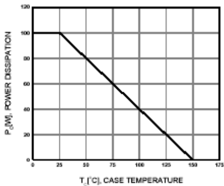
Figure 8. Power Derating
