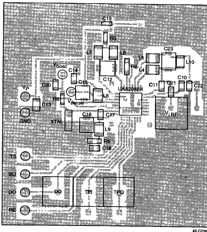
Fig.17 PCB top view with components for TQFP32; test circuit Fig.5.
