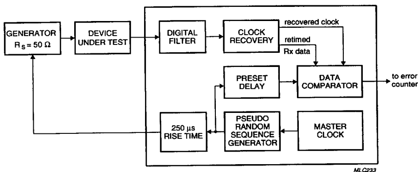
Fig.12 BER test facility.
