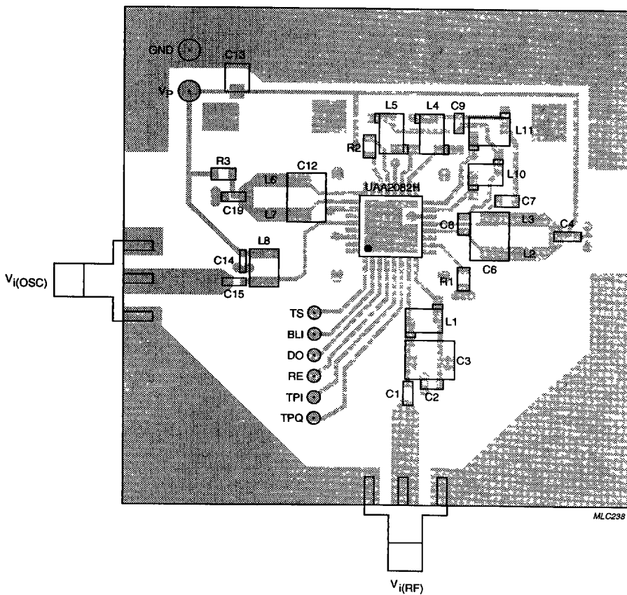
Fig.19 PCB top view with components for TQFP32; test circuit Fig.6.
