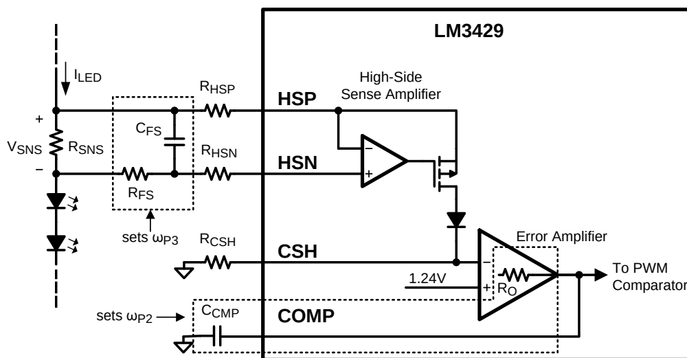
Figure 21. Compensation Circuitry
