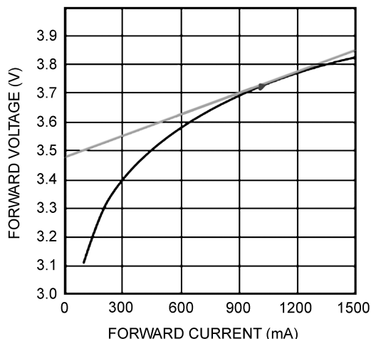
Figure 27. Dynamic Resistance
