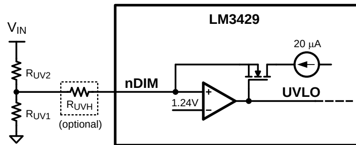
Figure 25. UVLO Circuit
