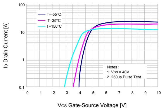
Figure 2. Transfer Characteristics
