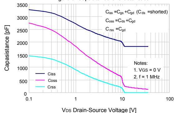
Figure 5. Capacitance Characteristics
