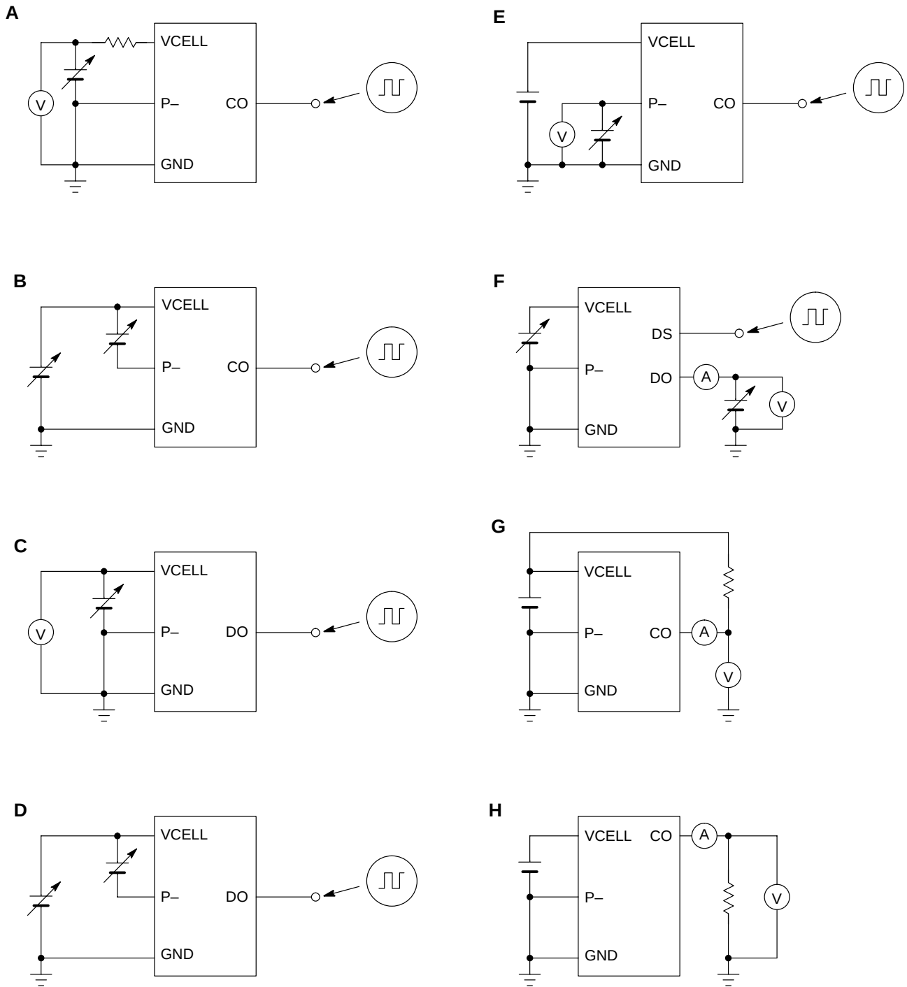
Figure 42. Test Circuits
