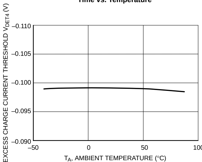
Figure 15. Excess Charge Current Threshold vs. Temperature
