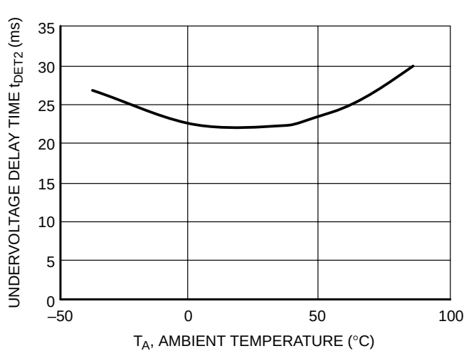
Figure 9. Undervoltage Delay Time vs. Temperature
