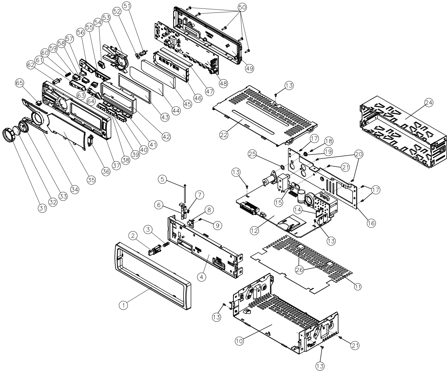
HS8003 4x7W EXPLODE DRAWING
