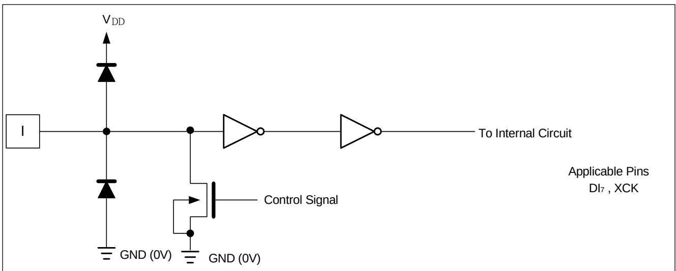
Figure 2 Input Circuit (2)
