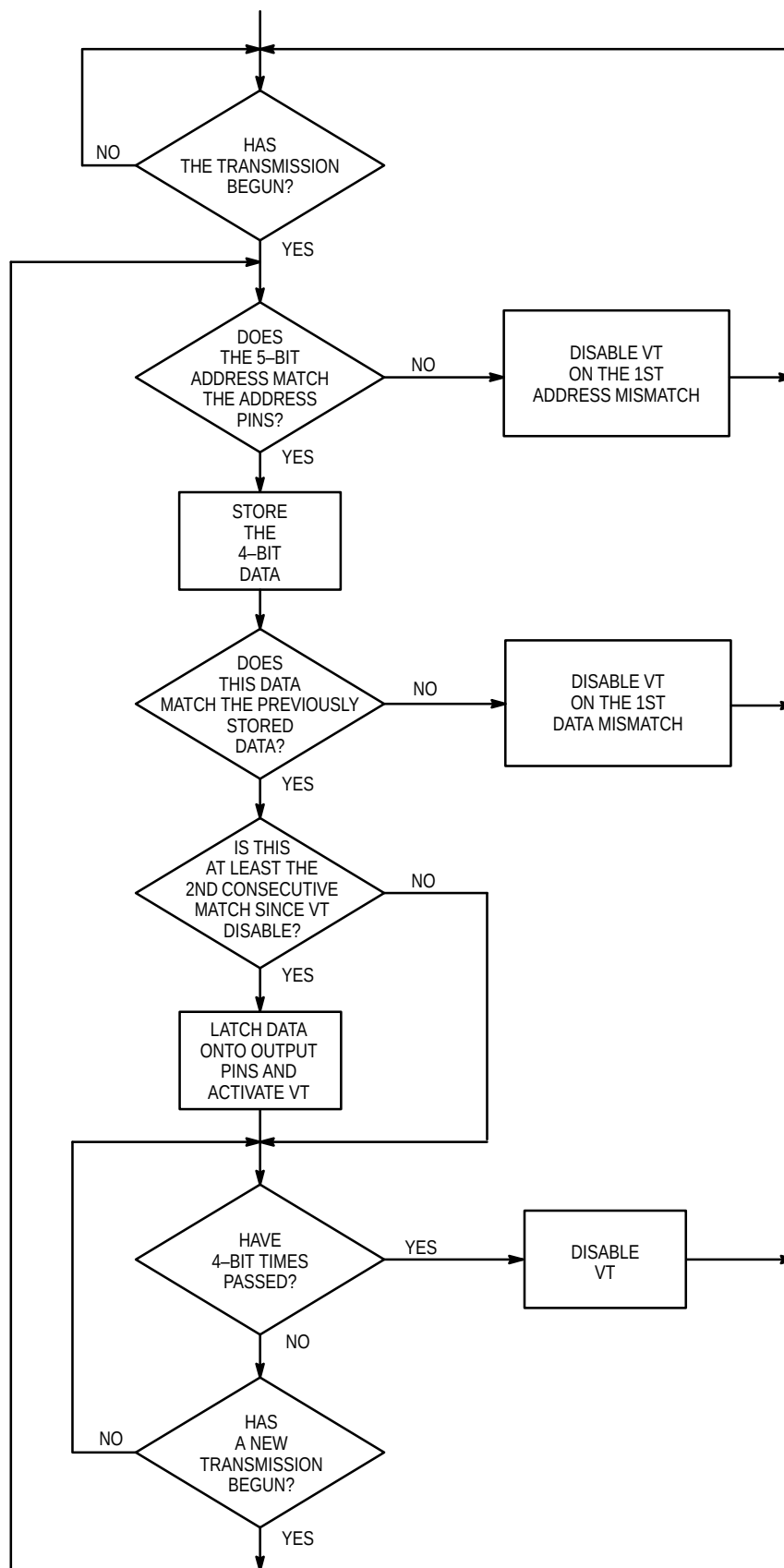
Figure 13. MC145027 Flowchart
