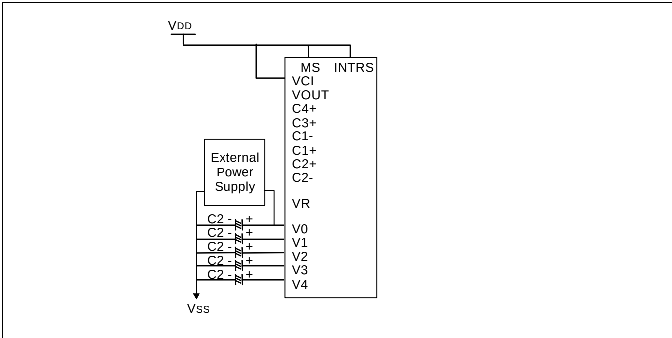
Figure 19. When Using some Internal LCD Power Circuits (VCI = VDD, VIC: OFF, VIR: OFF, VIF: ON)
