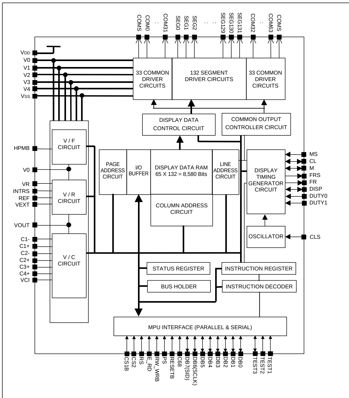
Figure 1. Block Diagram
