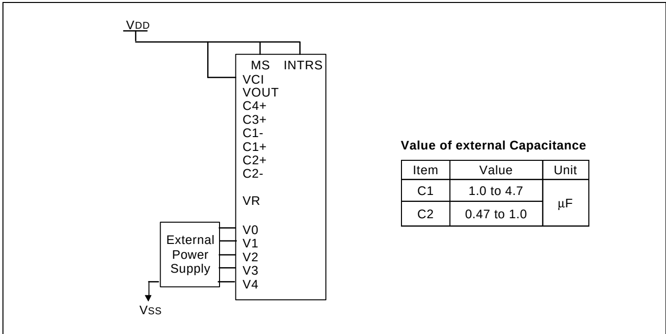
Figure 20. When not Using any Internal LCD Power Supply Circuits (VCI = VDD, VIC: OFF, VIR: OFF, VIF: OFF)
