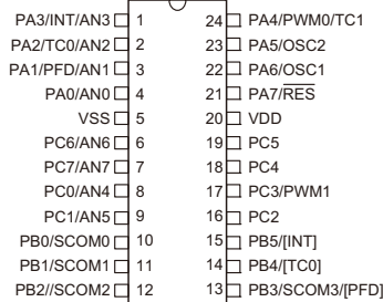
HT46R066 24 SKDIP-A/SOP-A/SSOP-A
