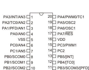
HT46R066 20 DIP-A/SOP-A/SSOP-A
