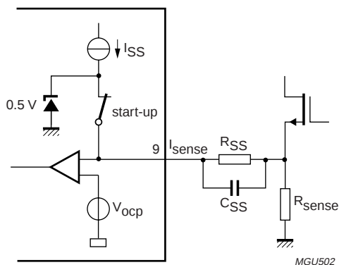
Fig.10 Soft start.
