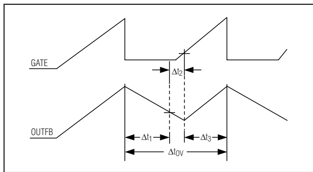
Figure 5. MAX6495/MAX6496/MAX6499 Timing
