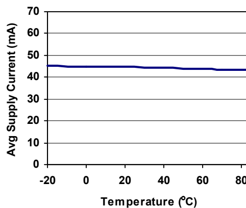
Supply Current vs. Ambient Temperature
