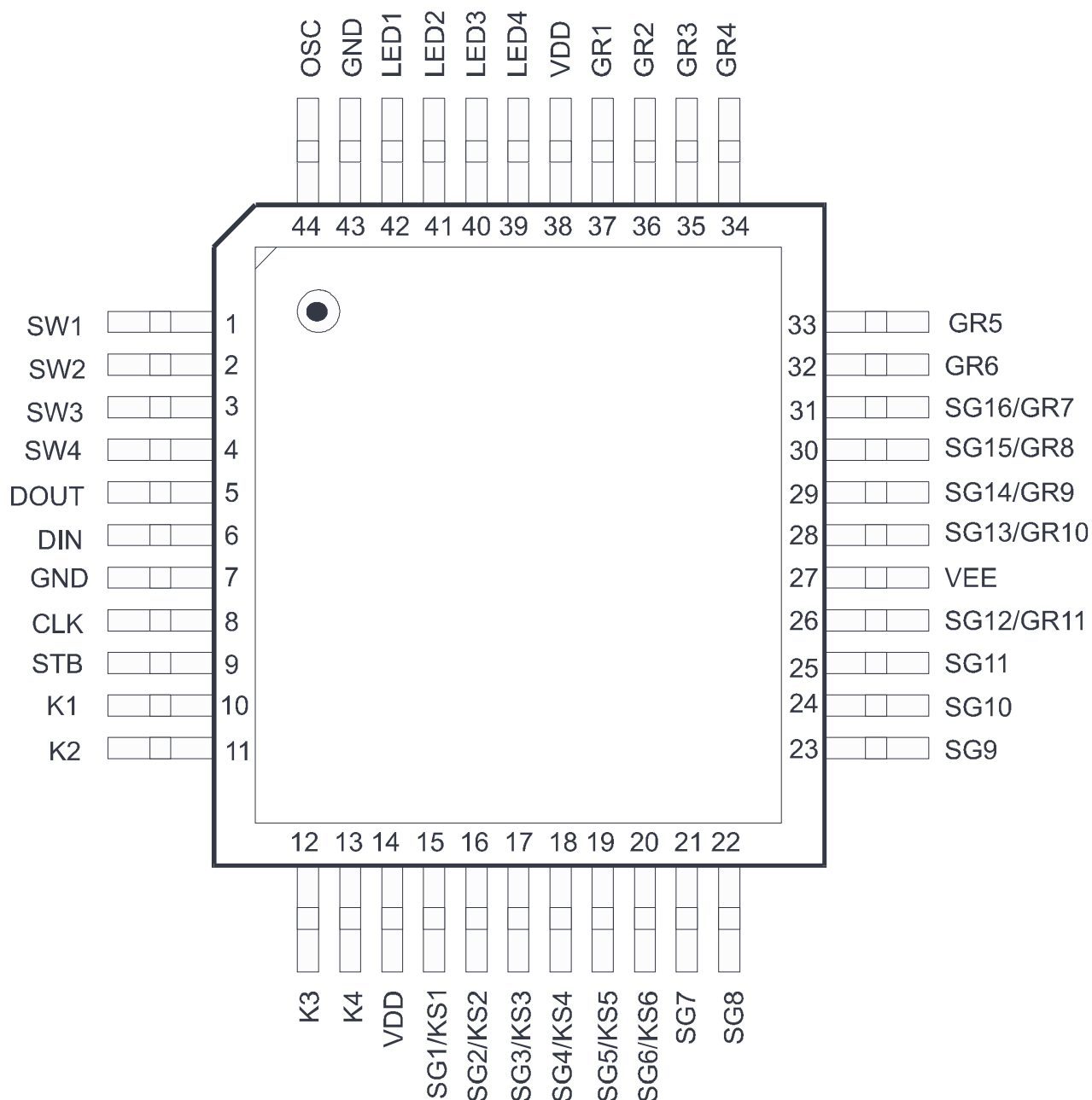
Figure 2: PT6312 Pin Configuration
