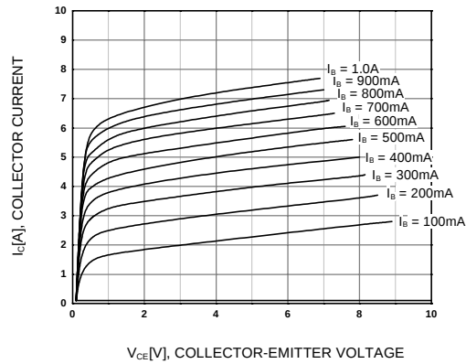
Figure 1. Static Characteristic
