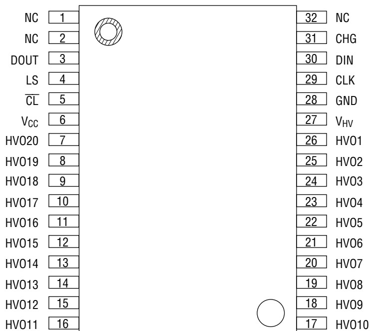
32-Pin Plastic SSOP
