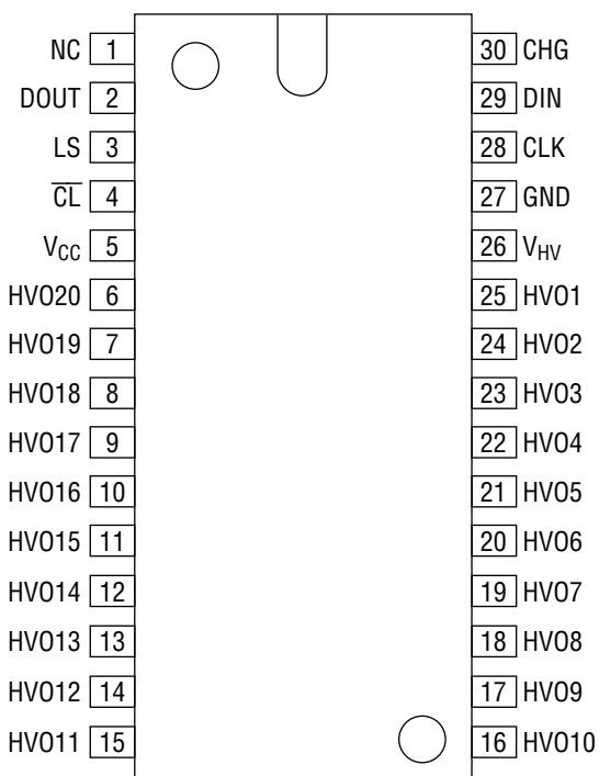
30-Pin Plastic Shrink DIP
