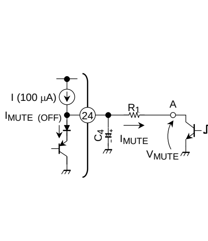
Figure 4 Muting Function
