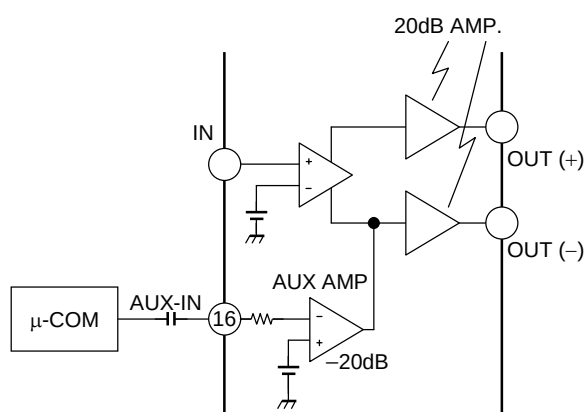
Figure 6 AUX Input
