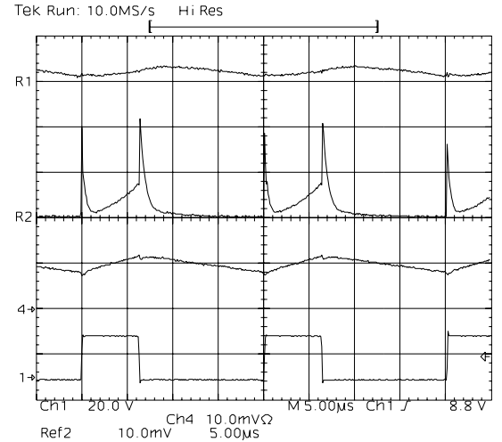
Figure 9: Waveforms in the experimental circuit using the coupled-inductor design #2; top-to-bottom: (R1) i_3 (100mA/div); (R2) i_2 (100mA/div); (4) i_1 (2A/div); (1) v_{s1} (20V/div). Operating conditions: V_{o1} = 5.1\text{V} , I_{o1} = 2\text{A} , V_{o2} = 5.7\text{V} , I_{o2} = 20\text{mA} , V_{o3} = 5.66\text{V} , I_{o3} = 20\text{mA} .
