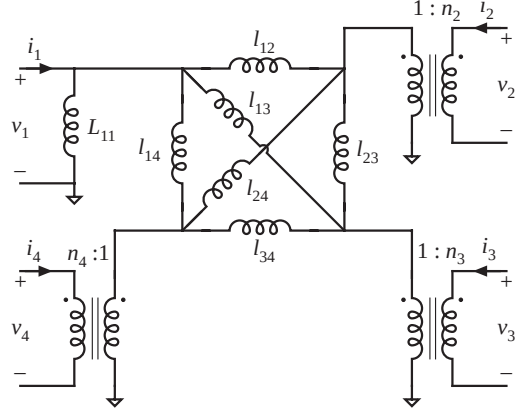
Figure 3: Extended cantilever model for 4 coupled inductors.
