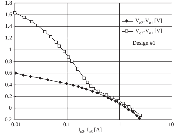
Figure 11: Experimental cross-regulation (V_{o2}-V_{o1})(I_{o2}) at I_{o1} = 2\text{A} , I_{o3} = 1\text{A} , and (V_{o3}-V_{o1})(I_{o3}) at I_{o1} = 2\text{A} , I_{o2} = 1\text{A} , using the coupled-inductor design #1.
