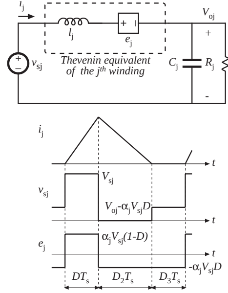
Figure 5: Equivalent circuit model of the j^{th} winding and waveforms used in the analysis of the discontinuous conduction mode.
