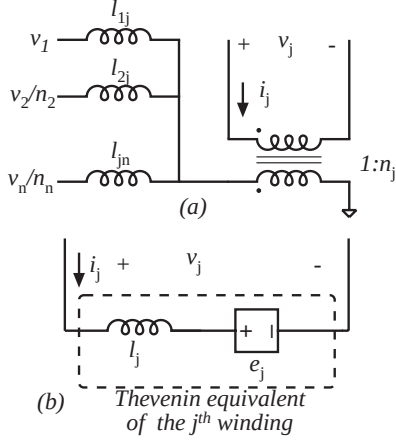
Figure 4: Derivation of the Thevenin equivalent circuit for the j^{th} winding.
