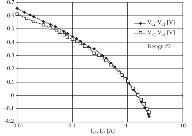
Figure 12: Experimental cross-regulation (V_{o2}-V_{o1})(I_{o2}) at I_{o1} = 2\text{A} , I_{o3} = 1\text{A} , and (V_{o3}-V_{o1})(I_{o3}) at I_{o1} = 2\text{A} , I_{o2} = 1\text{A} , using the coupled-inductor design #2.
