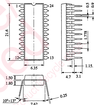
24-Lead Shrink DIP Plastic Package (24-SDIP)
