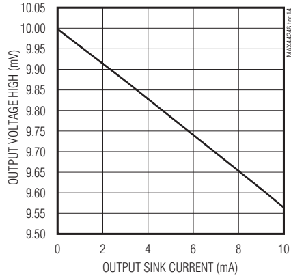
OUTPUT VOLTAGE HIGH vs. OUTPUT SINK CURRENT
