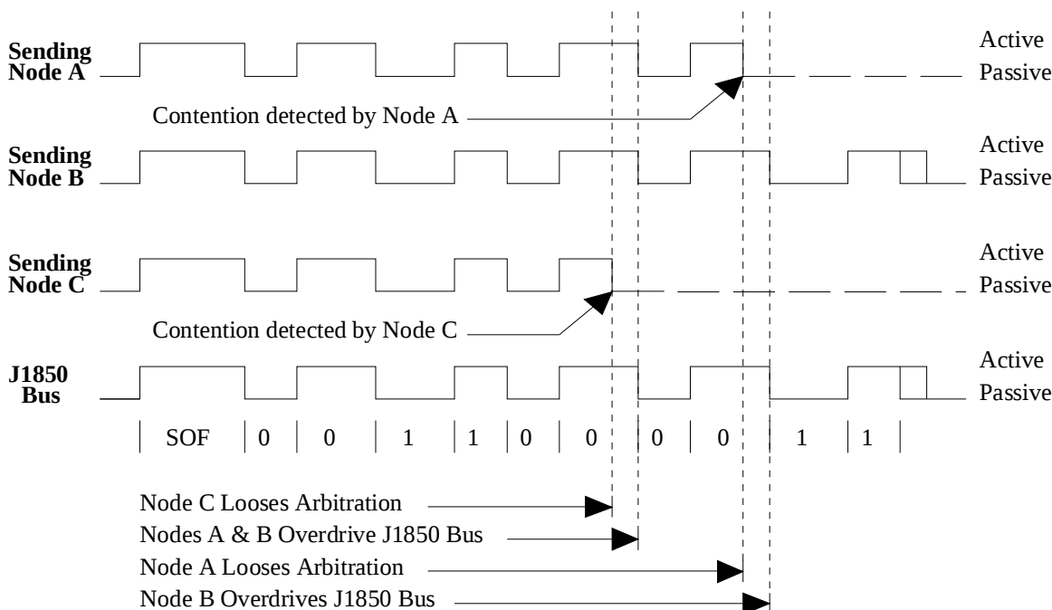
Figure 2. Bit-by-bit Arbitration
