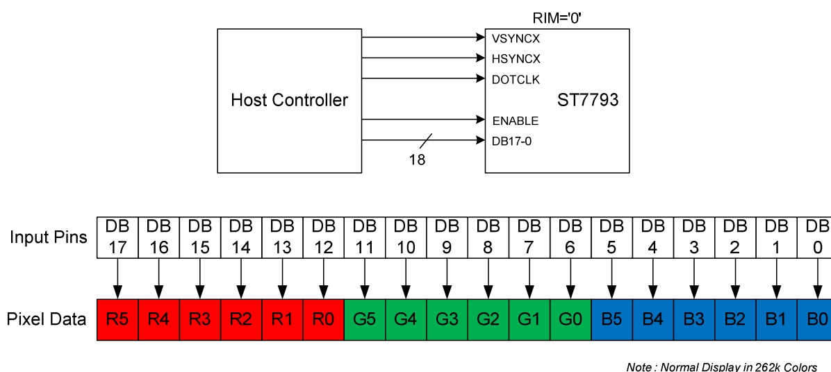
Figure 26 18-bit RGB Interface Data Format
