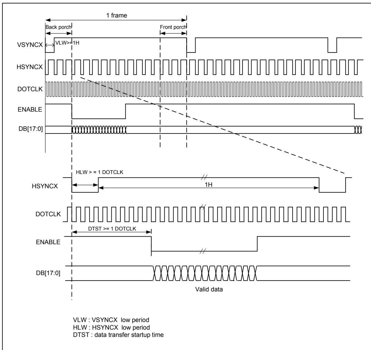
Figure 23 18-/16-bit RGB Interface Signal Relationship
