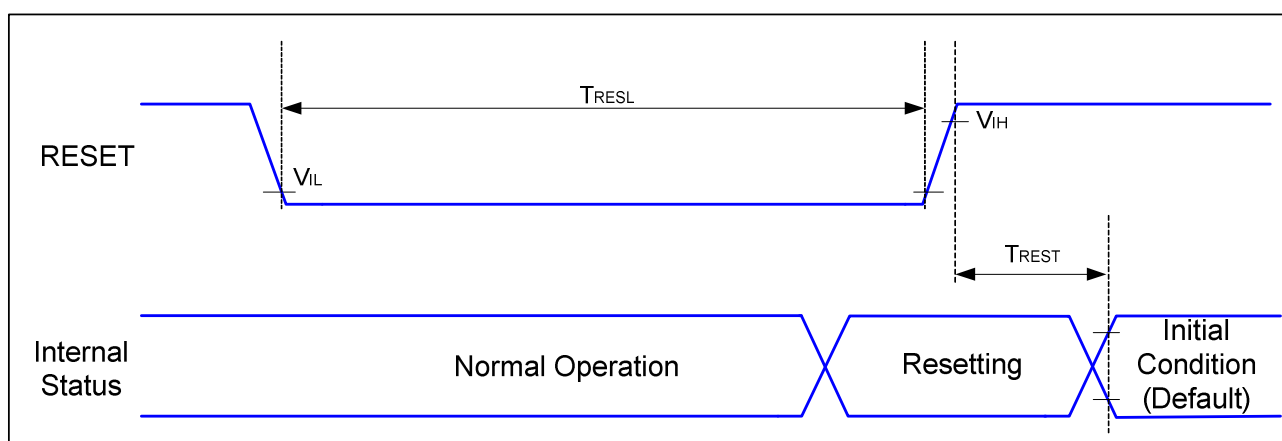
Figure 41 Reset Timing
