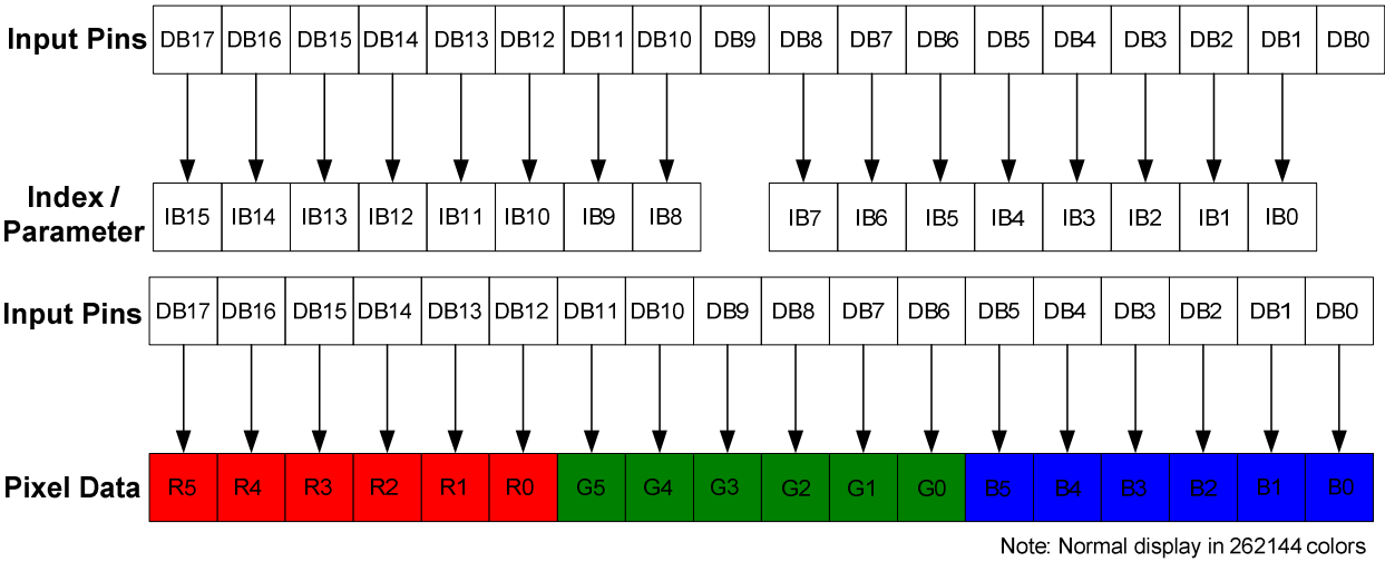
Figure 9 18-bit 8080-Series Interface Data Format (Index/Parameter/Pixel Data Write)
