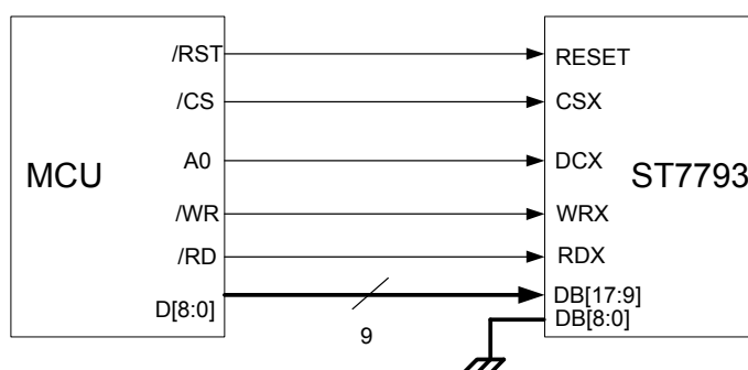
Figure 12 9-bit 8080-Series Interface Connection
