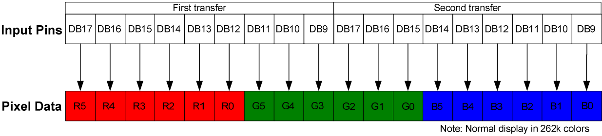
Figure 13 9-bit 8080-Series Interface Data Format (Index/Parameter/Pixel Data Write)
