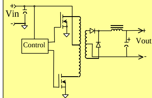
Simplified Schematic
