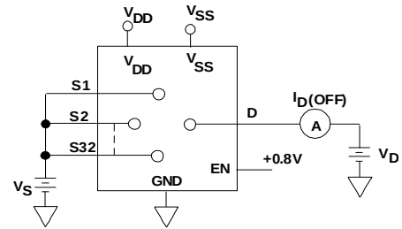
Test Circuit 3. I_D (OFF)
