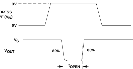
Test Circuit 6. Break Before Make Delay, t_{OPEN} .
