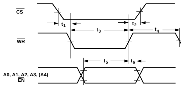
Figure 1. Timing Diagram
