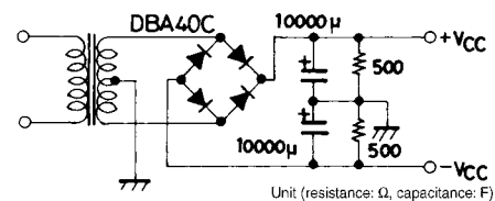
Specified Transformer Power Supply (Equivalent to MG-200)
