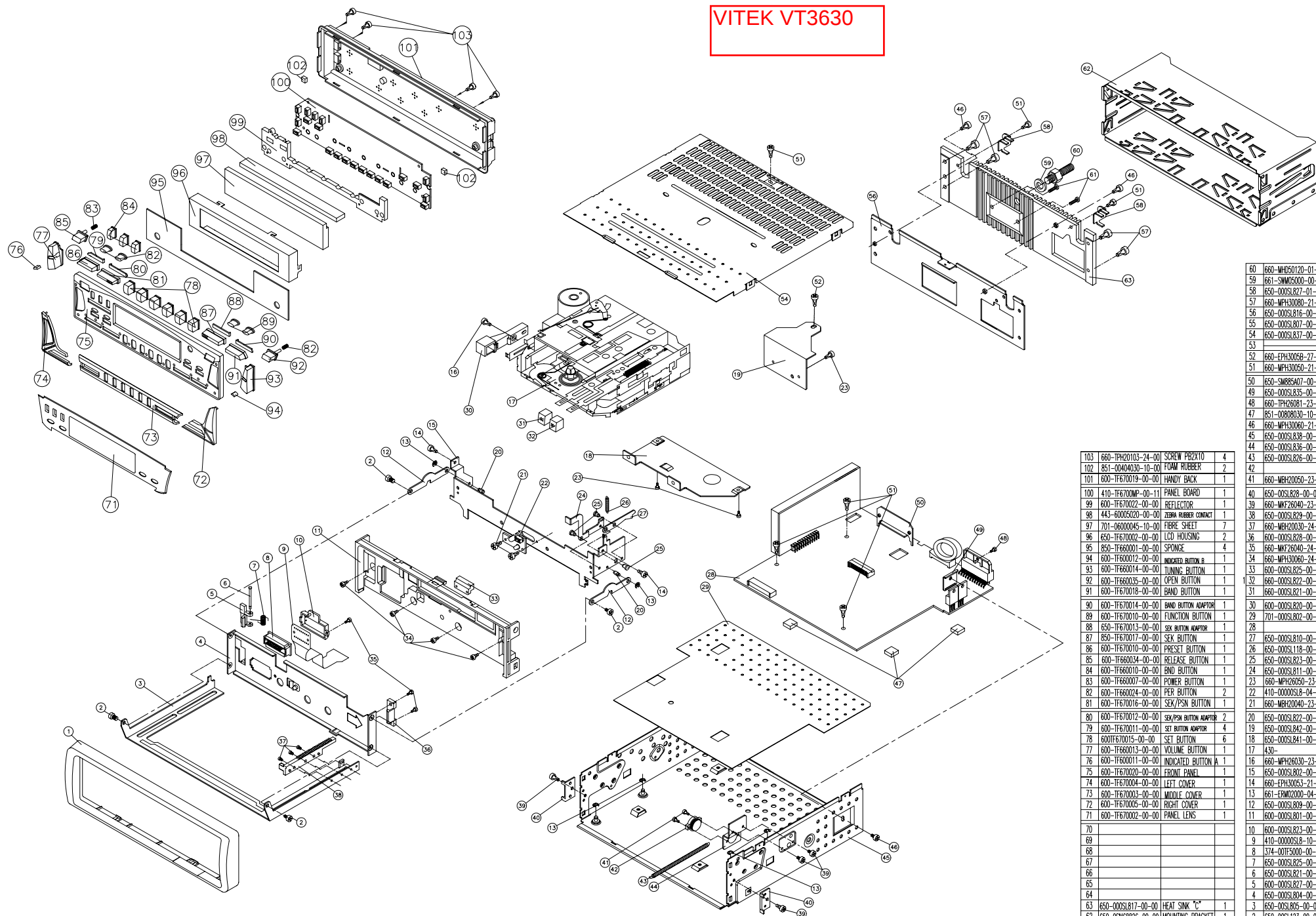
VITEK VT-3630 EXPLODED
