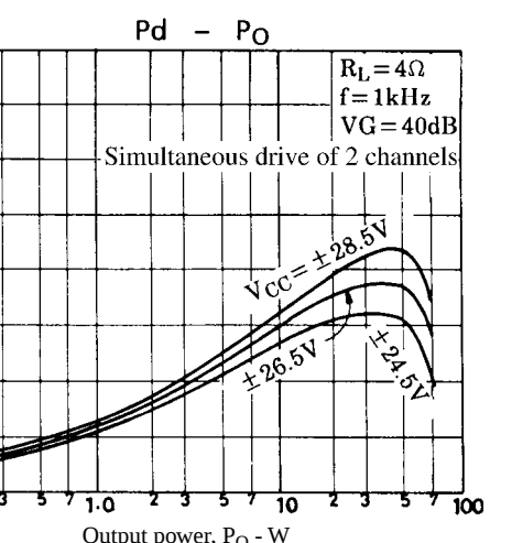
Figure 2. STK4161V Pd – P_O ( R_L = 4\Omega )
