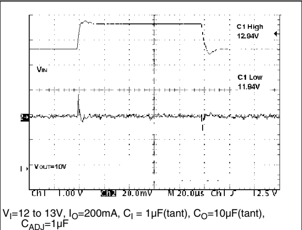
Figure 21. Line transient
