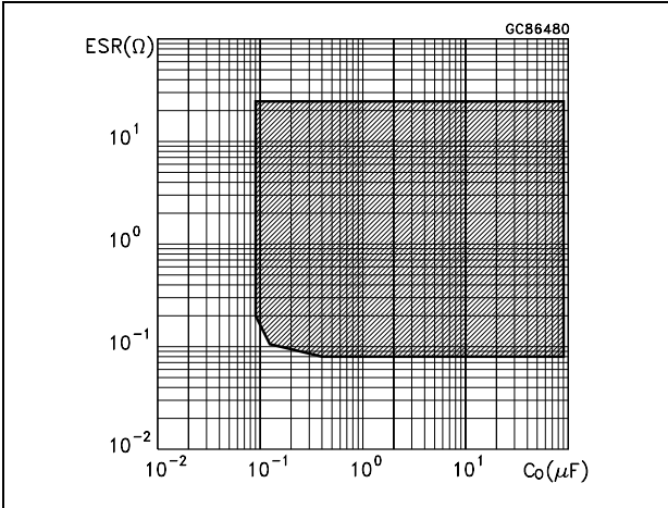
Figure 20. Stability
