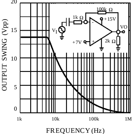
OUTPUT CHARACTERISTICS
