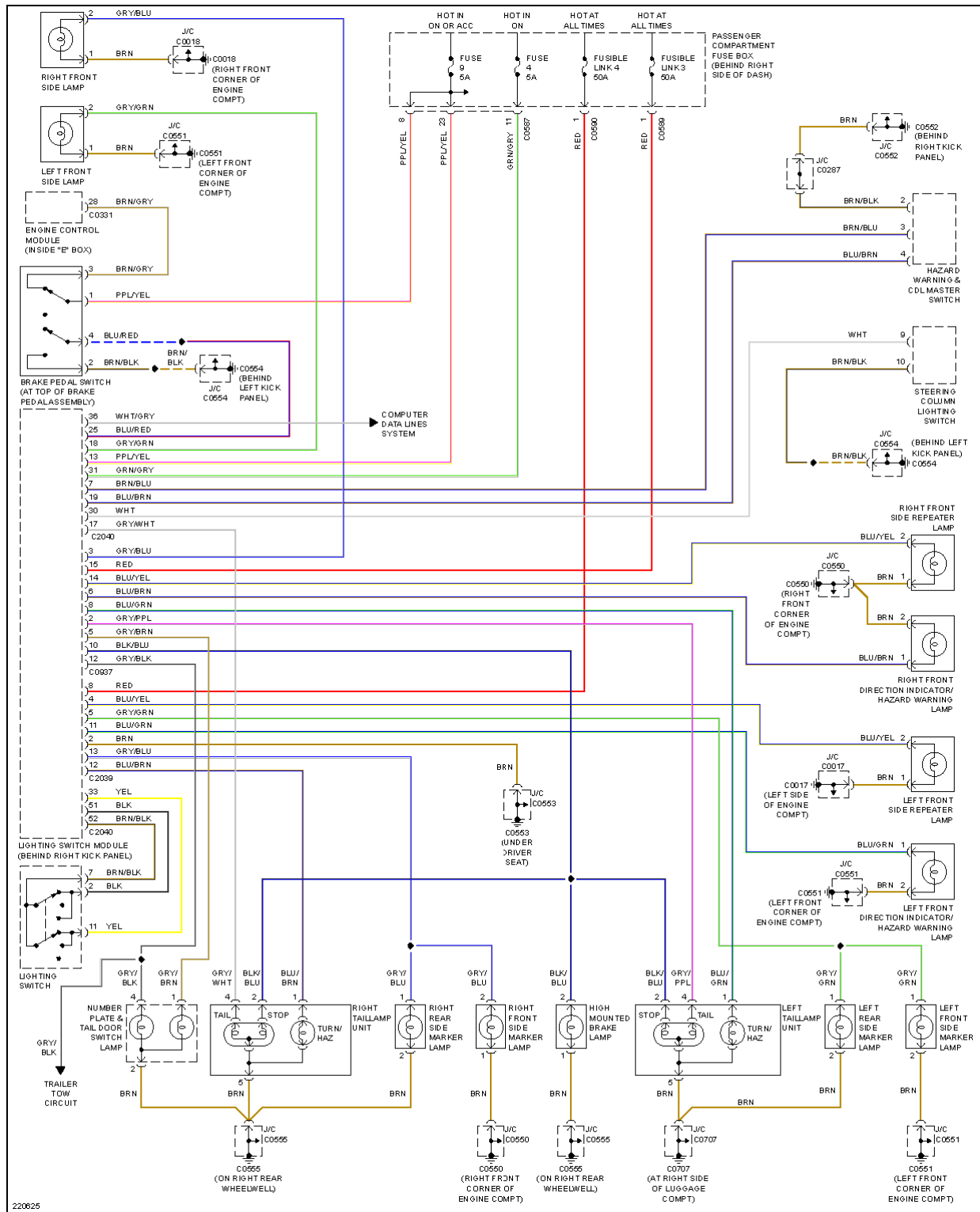
Fig. 23: Exterior Lamps Circuit
