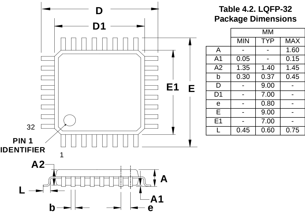
Figure 4.3. LQFP-32 Package Diagram
