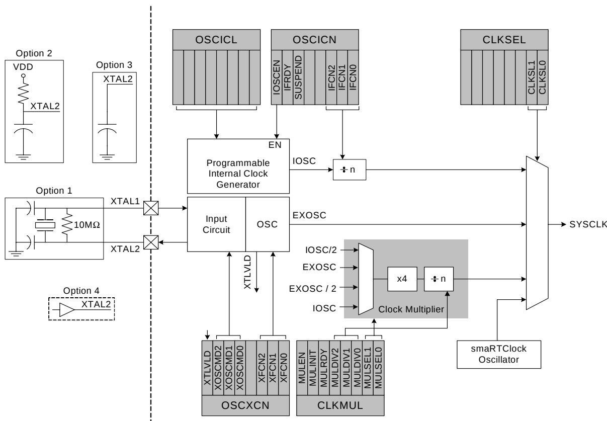
Figure 19.1. Oscillator Diagram
