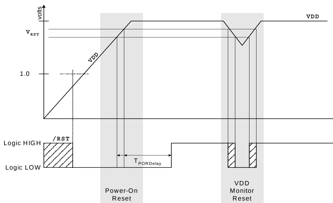
Figure 15.2. Power-On and V_{DD} Monitor Reset Timing
