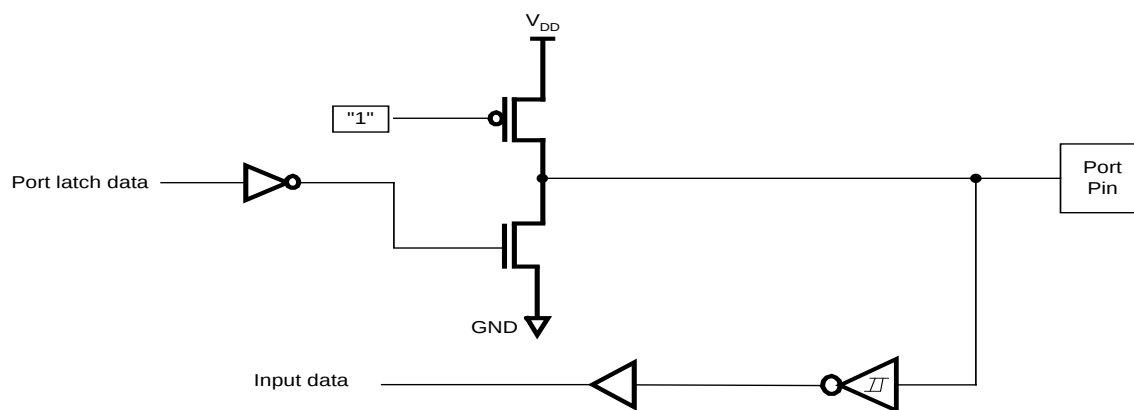
Open-Drain Mode
