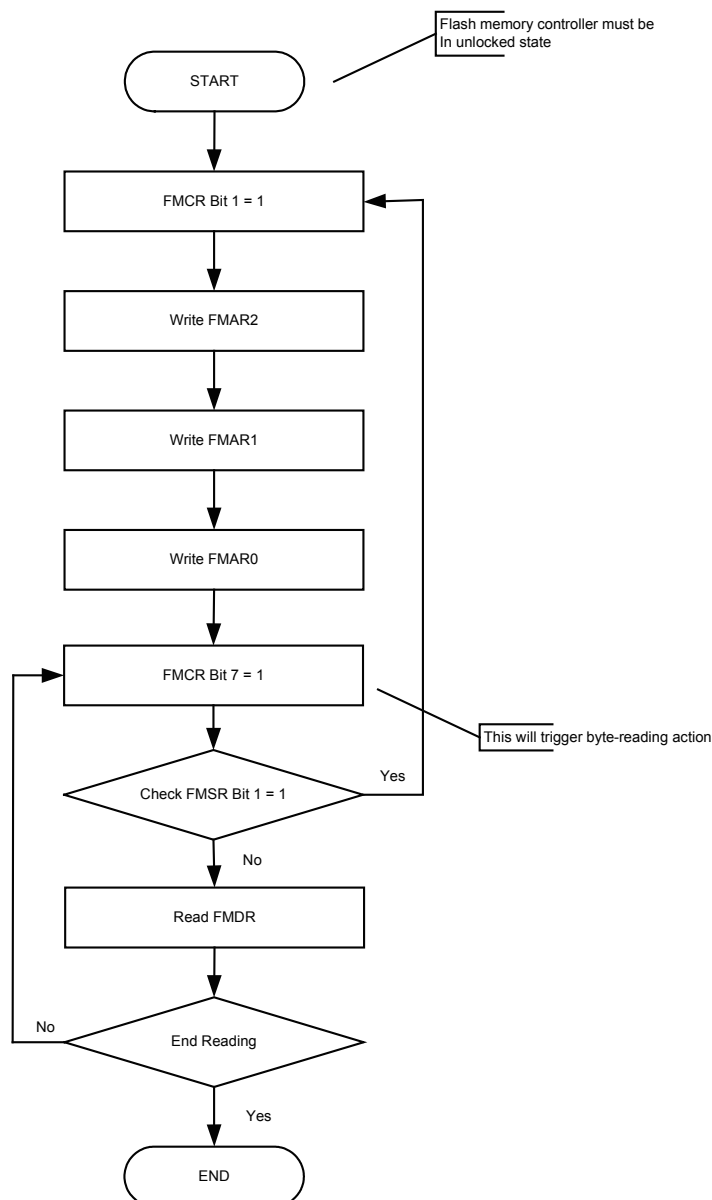
Byte Read Flowchart
