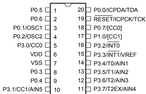
HT85F2240/HT85F2230/HT85V2240 20 DIP-A/SOP-A/SSOP-A
