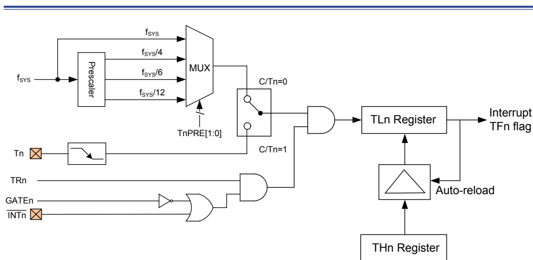
Mode 2 Block Diagram – Timer 0, 1
