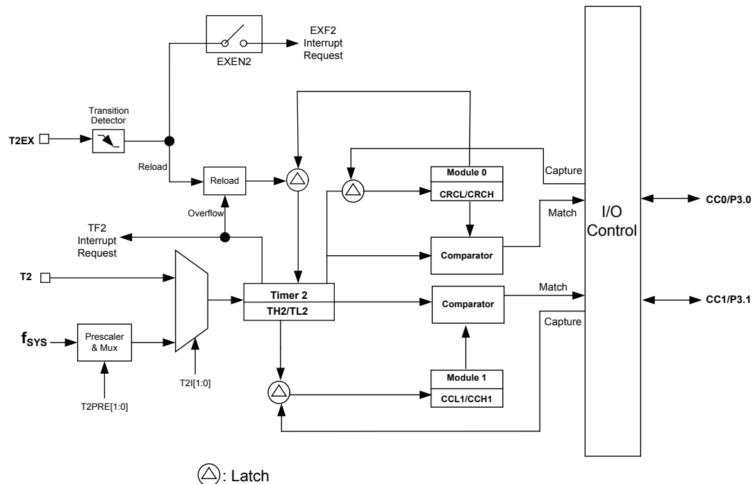
Timer 2 with PCA Modules Block Diagram
