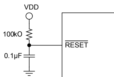
Basic Reset Circuit
