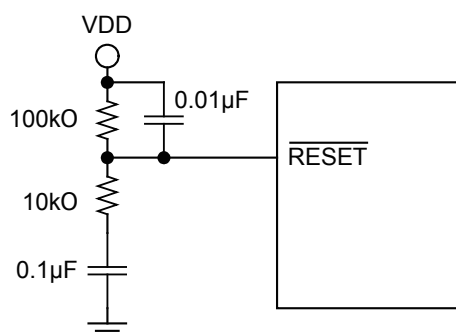
Enhanced Reset Circuit
