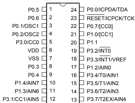
HT85F2240/HT85V2240 24 SKDIP-A/SOP-A/SSOP-A
