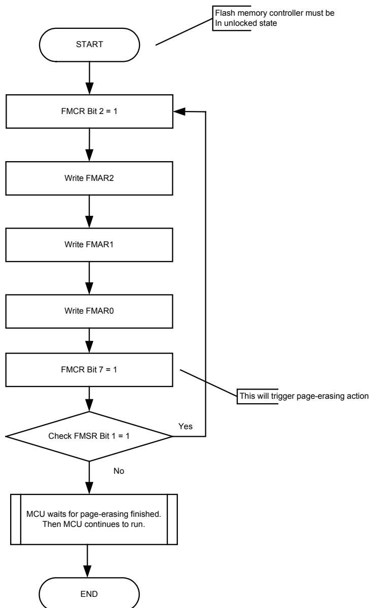
Page Erase Flowchart
