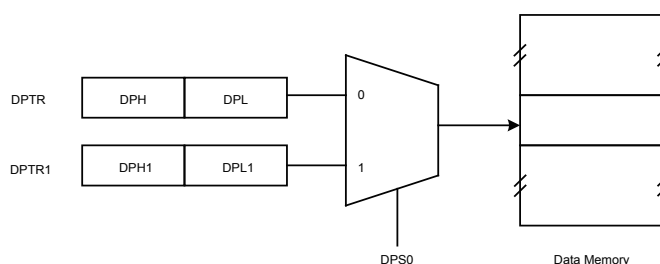
DPTRn Registers Control Block Diagram
