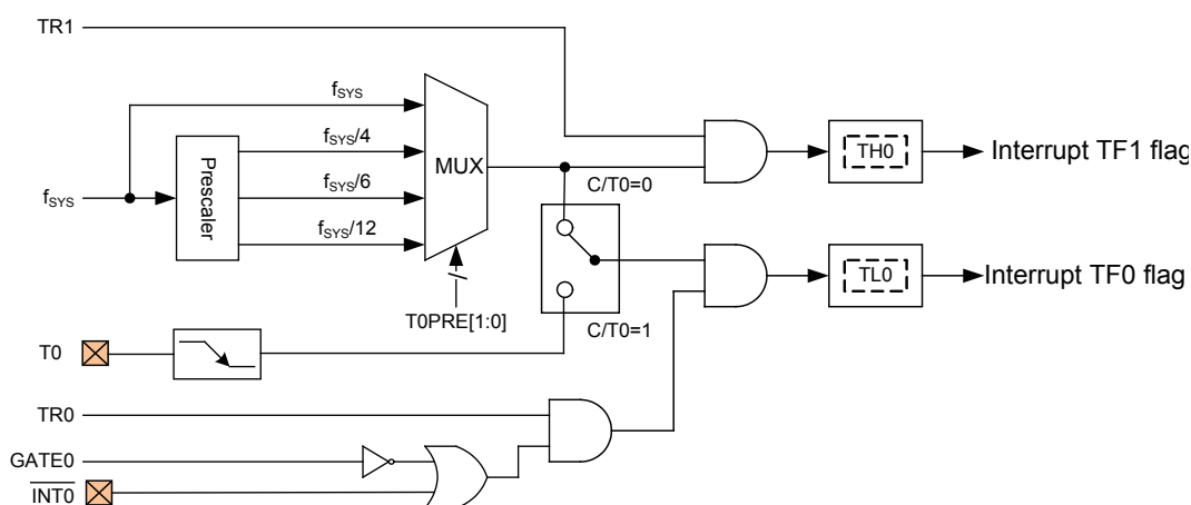
Mode 3 Block Diagram – Timer 0
