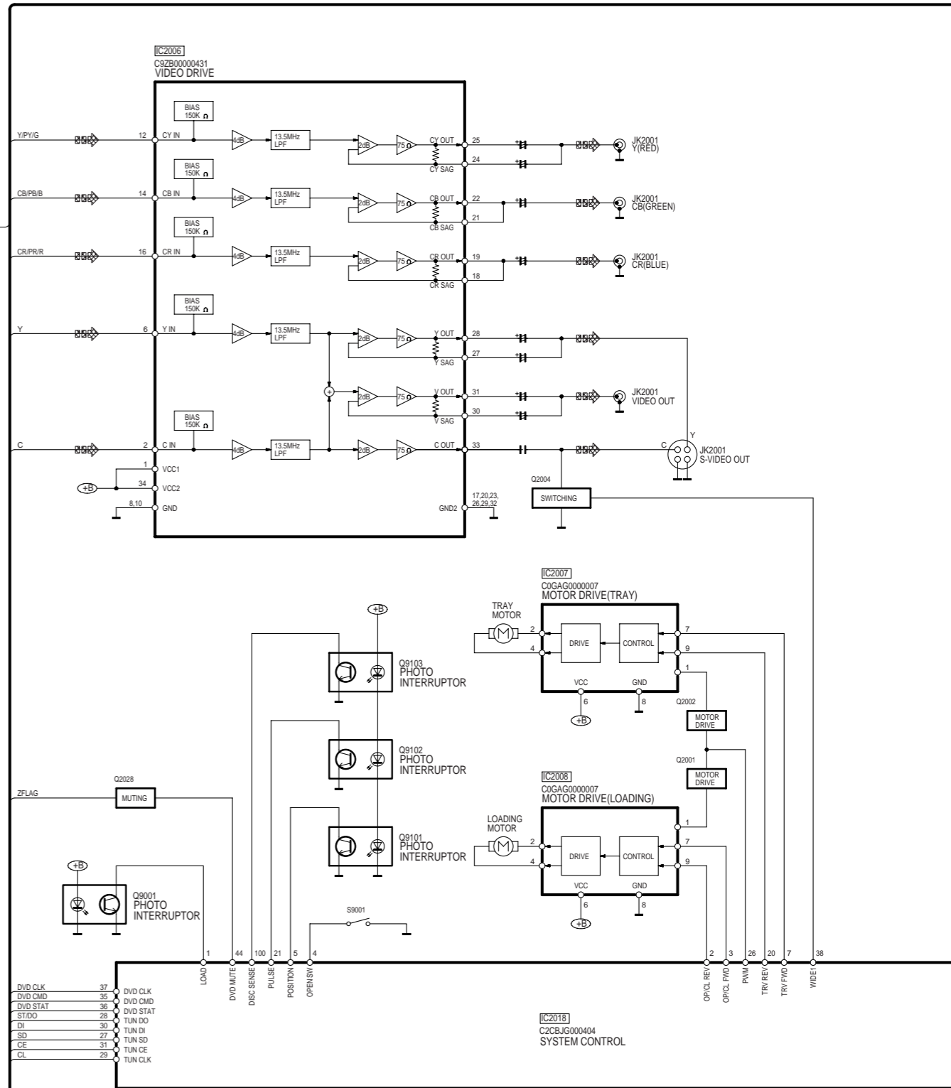
SA-HT928GC, GCS BLOCK DIAGRAM
