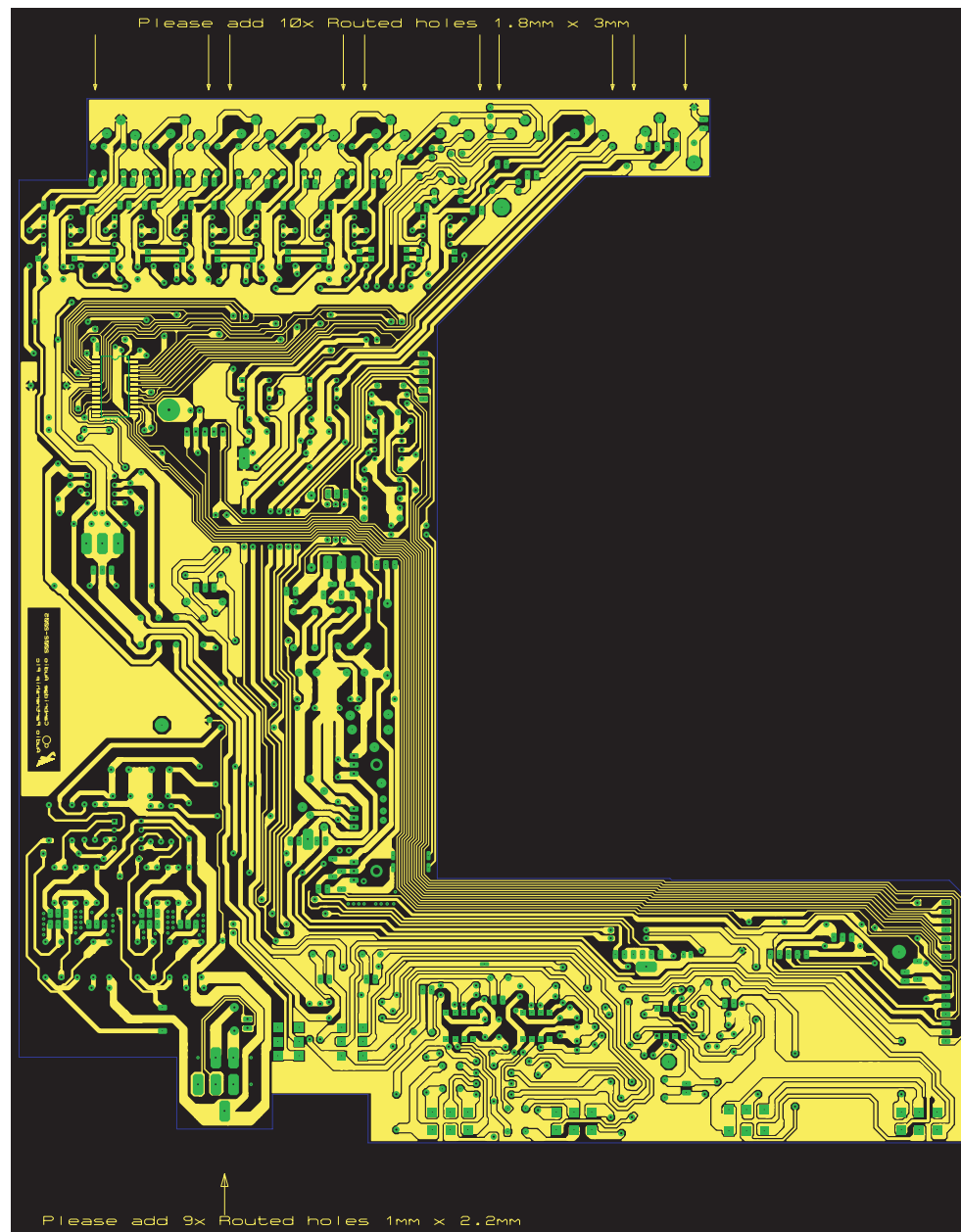
API 7649/4 Input PCB Board Layout (Bottom Side)
