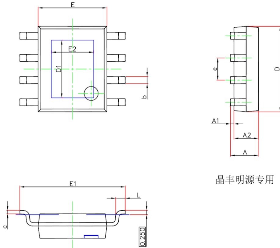
SOP8-EP (EXP PAD) PACKAGE OUTLINE DIMENSIONS
