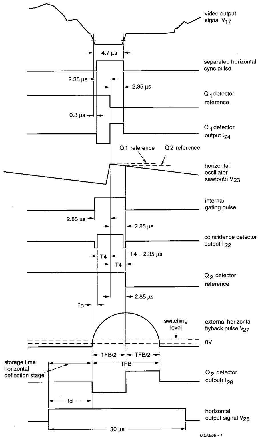
Fig.9 Timing diagram.
